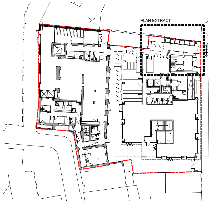
SITE PLAN LOCATION 1:500
