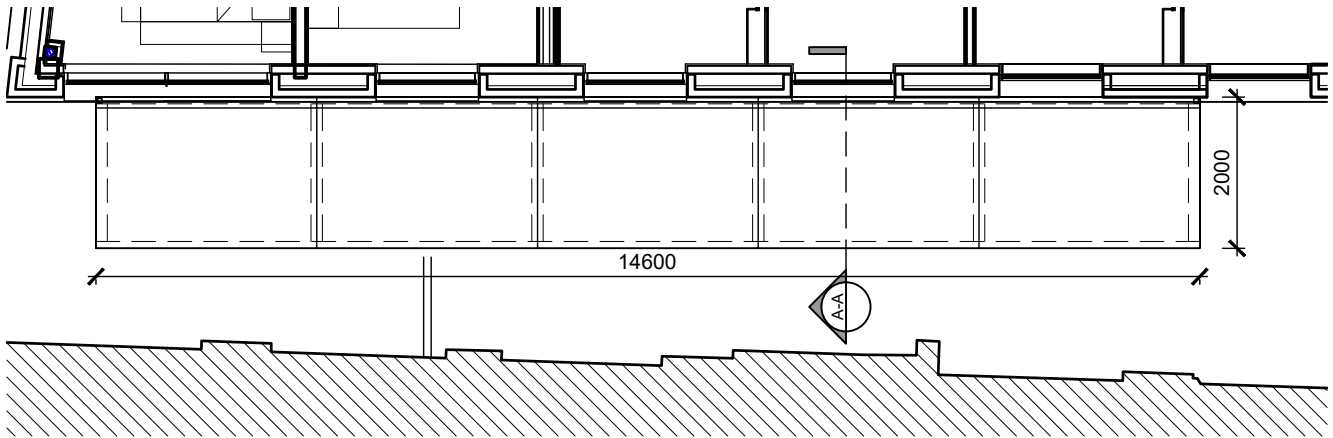
ROOF PLAN - 1:100
