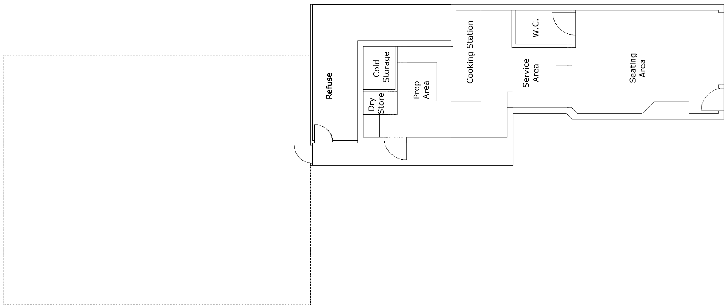
FLOORPLAN 1:100@A3
