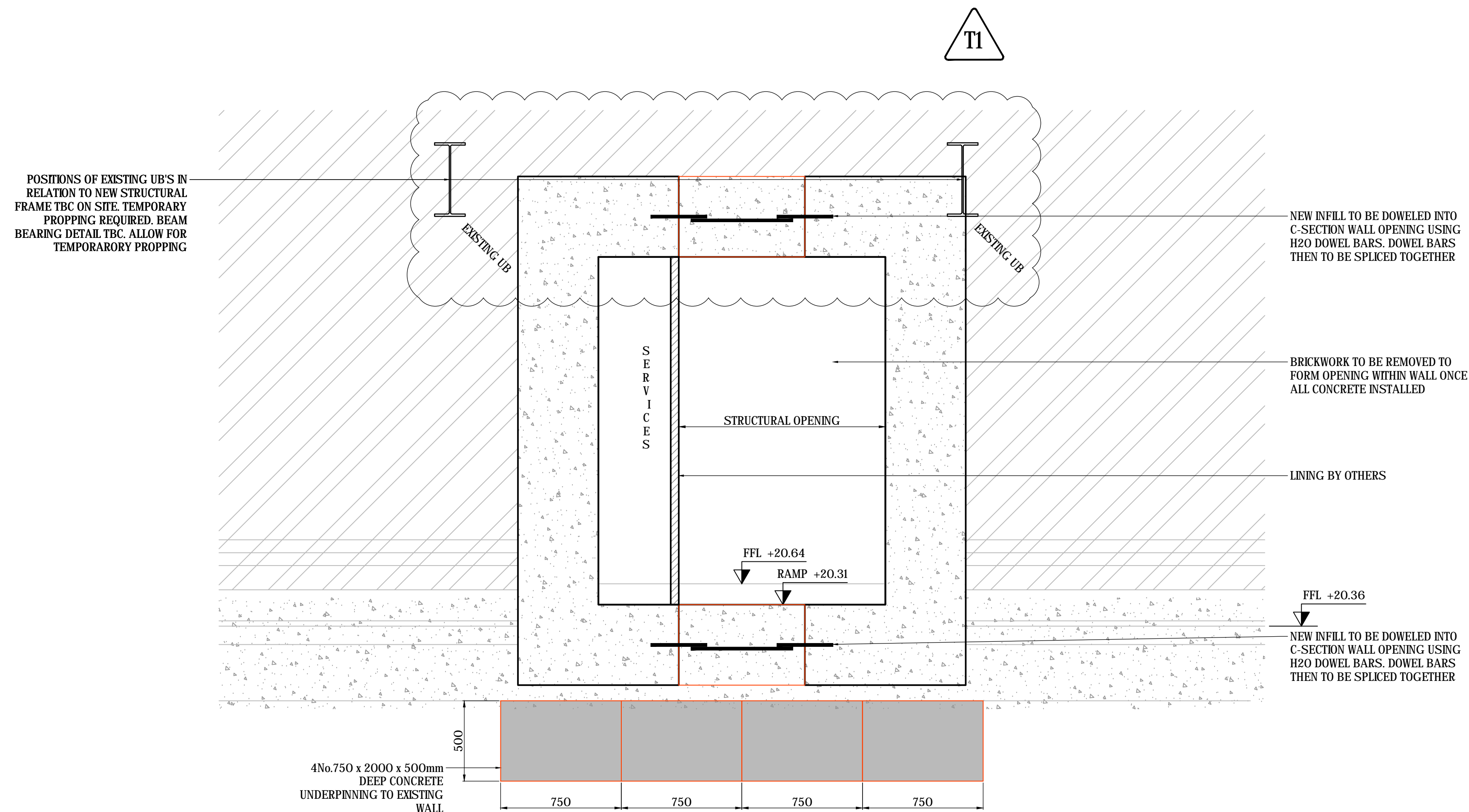
STEP 5 - TYPICAL ELEVATION ON OPENING (SCALE 1:20 AT A1)
