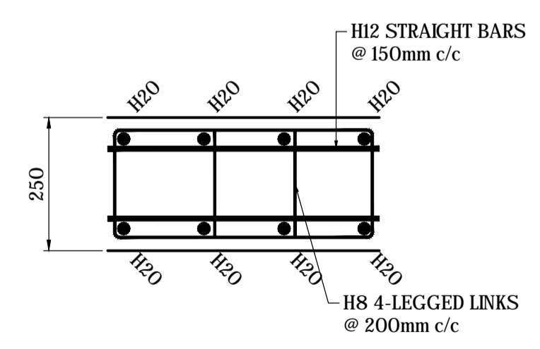
SECTION X-X (SCALE 1:10 AT A1)
