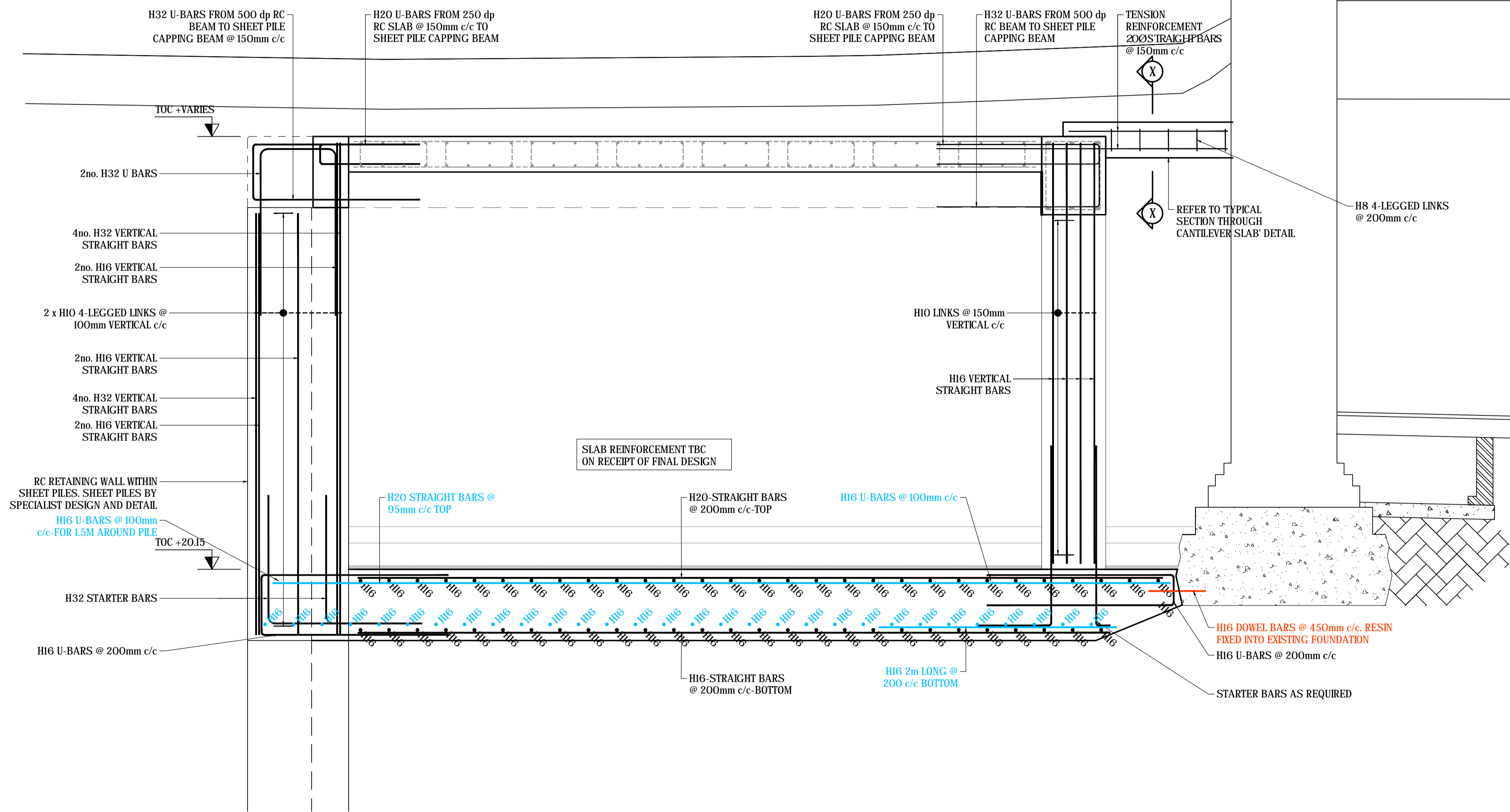
TYPICAL RC SECTION THROUGH BASEMENT BOX (SCALE 1:20 AT A1)
