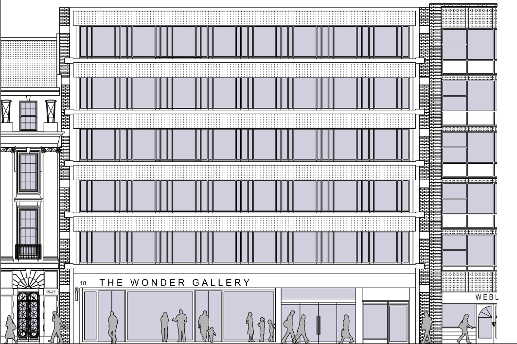
FRONT ELEVATION
