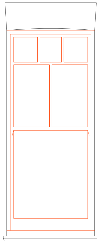
TYPICAL FACE OF SASH WINDOW SCALE 1:20
