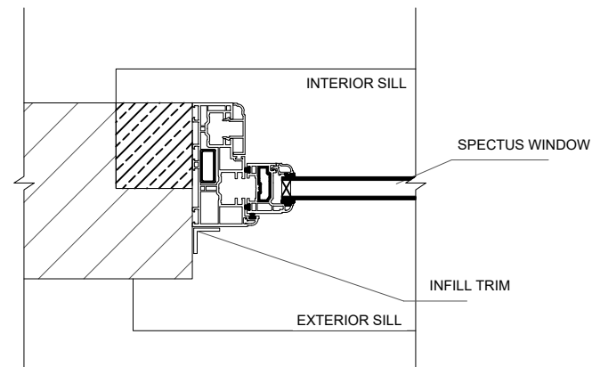
TYPICAL DOUBLE GLAZED uPVC WINDOW DETAIL SCALE 1:10
