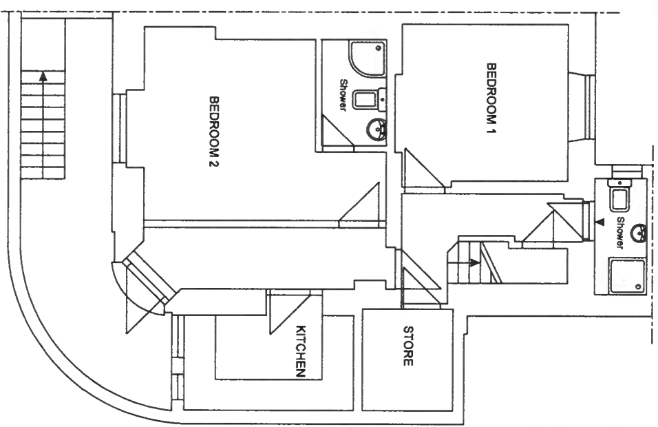
EXISTING BASEMENT FLOOR PLAN WITH ALTERATIONS SCALE 1/100
