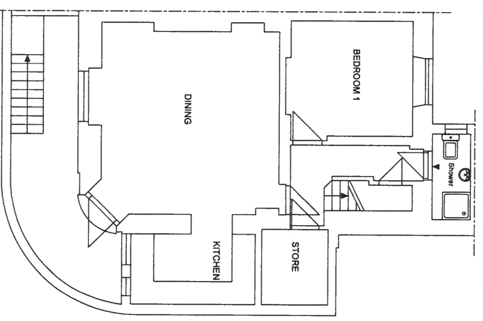
ORIGINAL BASEMENT FLOOR PLAN SCALE 1/100
