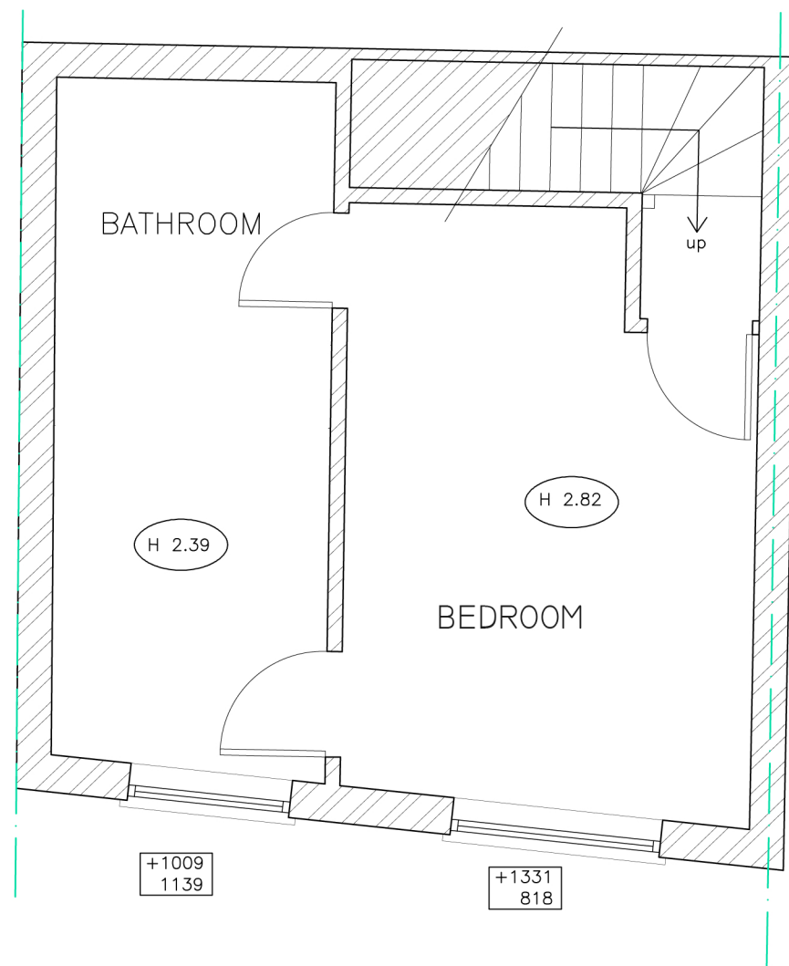
FIRST FLOOR SCALE 1:50
