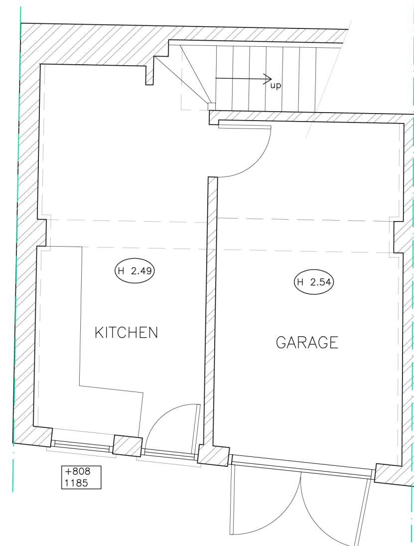
GROUND FLOOR SCALE 1:50
