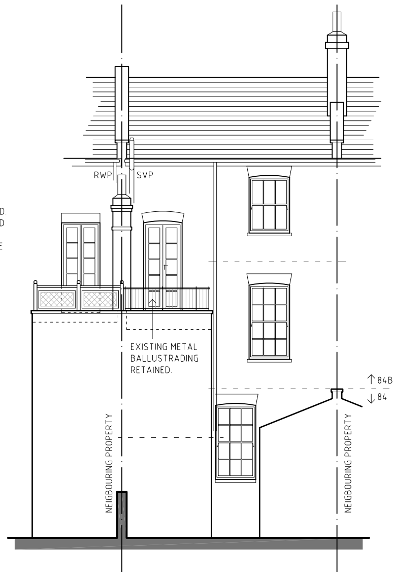
South Elevation
