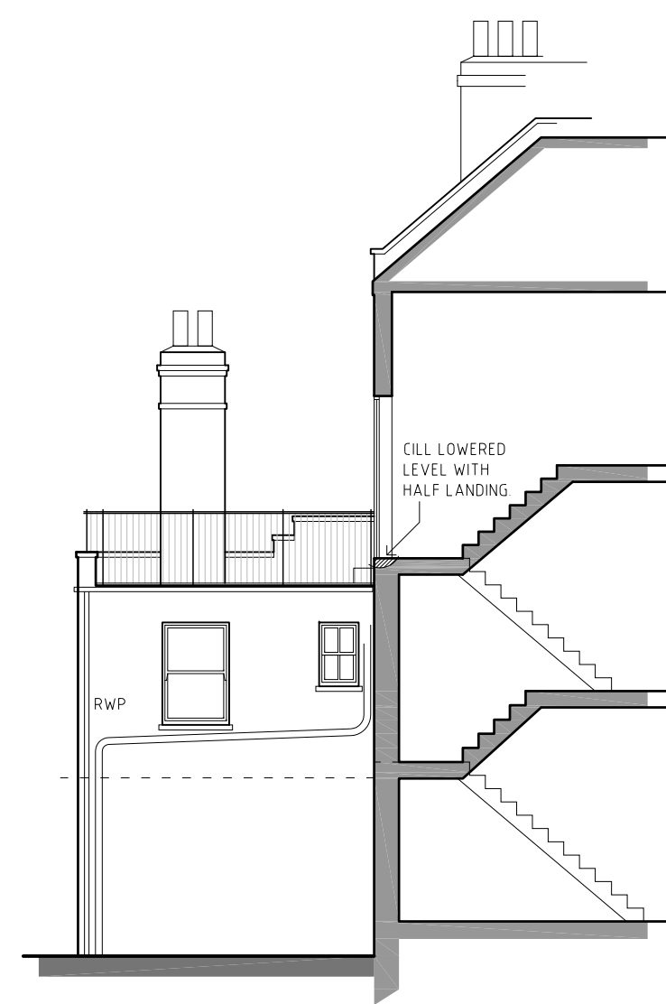
East Elevation
