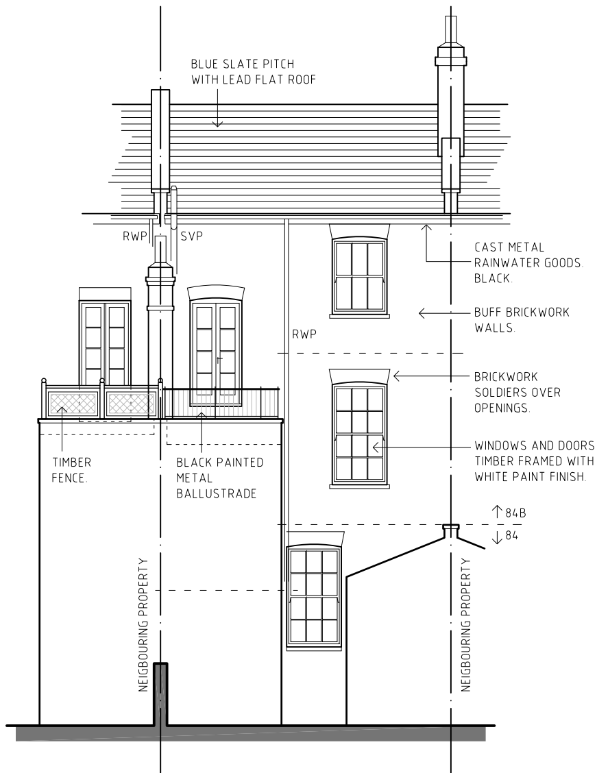
South Elevation
