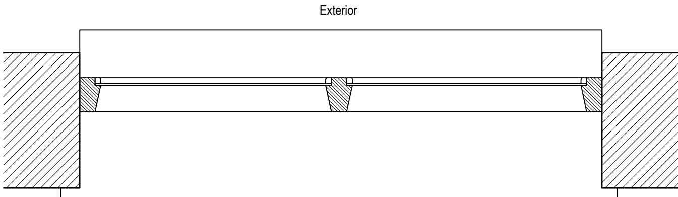
Section B-B
