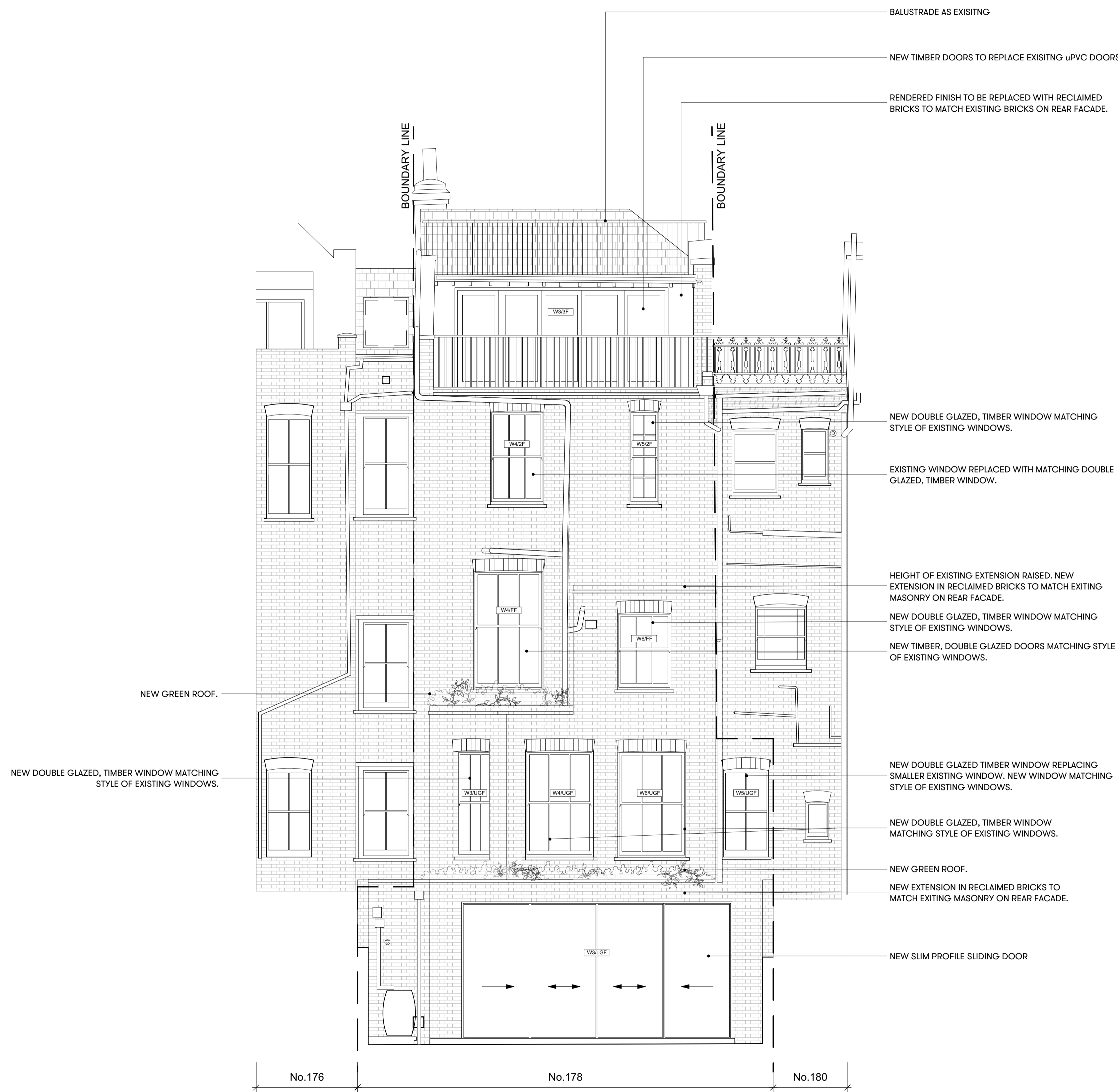
1 Proposed Rear Elevation Scale: 1:50-A1 / 1:100-A3
