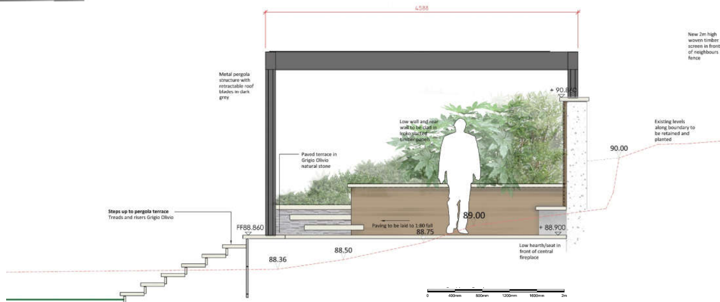
Left: Section AA through centre of pergola terrace – red dashed line shows existing ground level.
