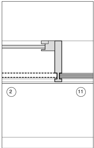
Facade To New Second Floor, 65 KCR
