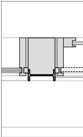
Plan Details
