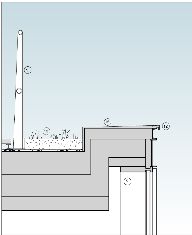
Section Through Edge of New Roof
