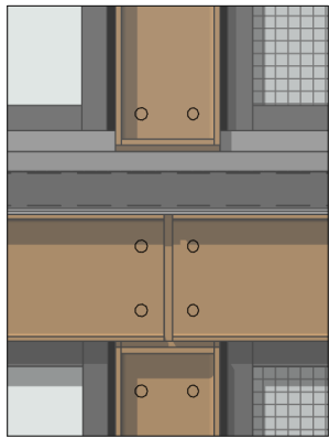
Elevation Details
