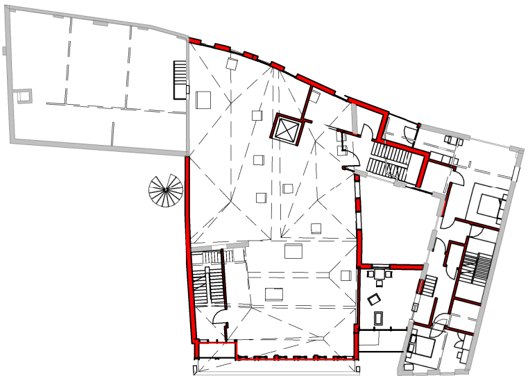
Second Floor
