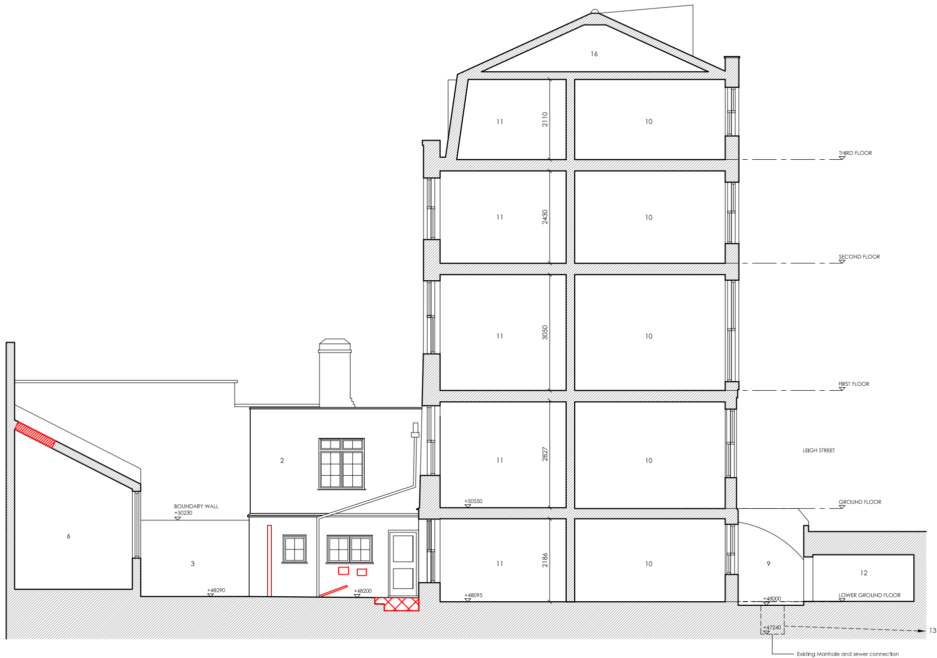
01 PL203 DEMOLITION SECTION AA SCALE 1:100 @ A3
