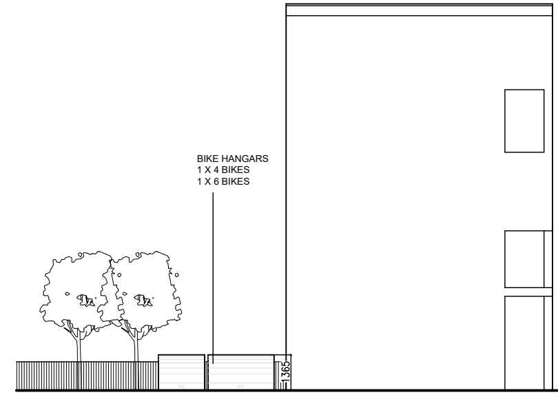
Proposed Elevation 04
