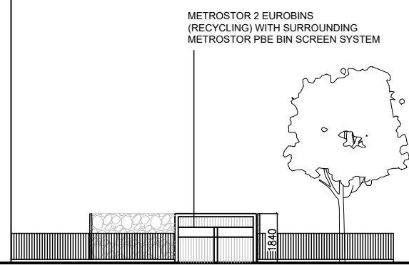
Proposed Elevation 06
