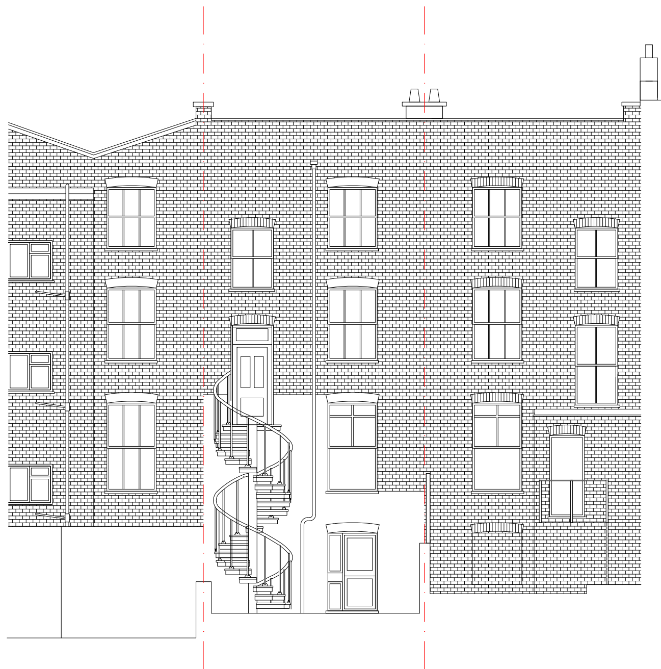
02 EXISTING REAR ELEVATION 1:200 @ A3
