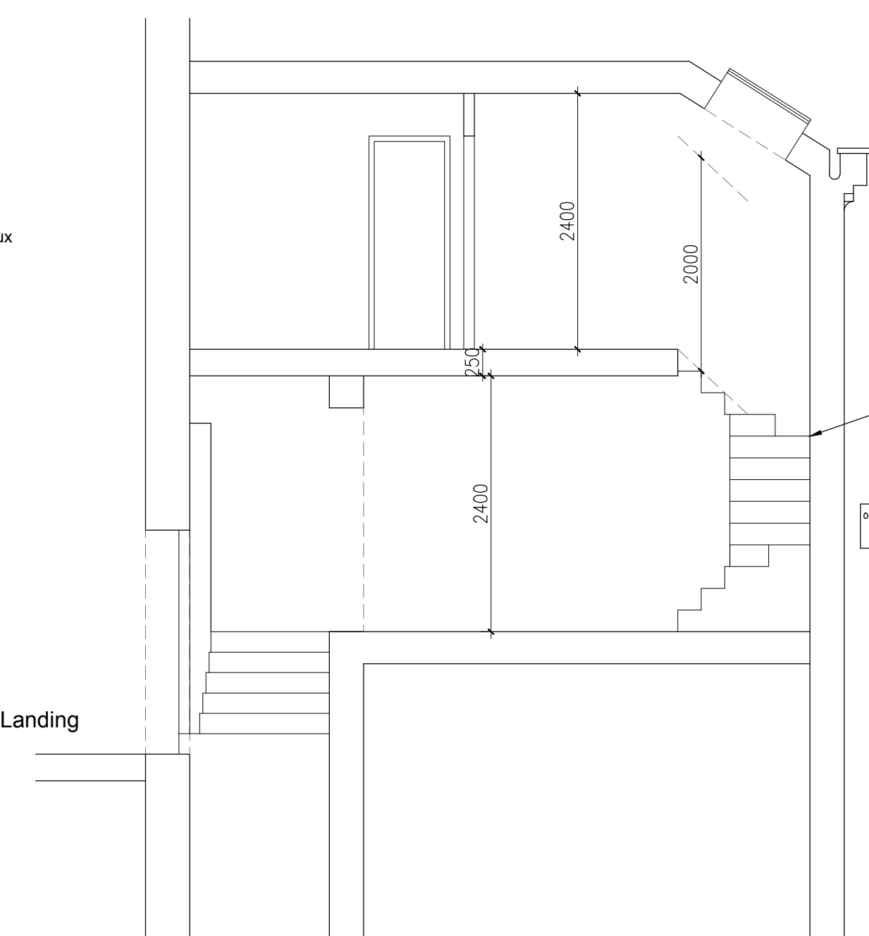
PROPOSED SECTION
