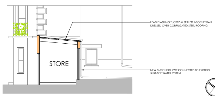
4 SIDE ELEVATION /SECTION PROPOSED 1:100
