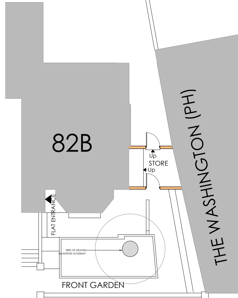
1 PLAN PROPOSED 1:100
