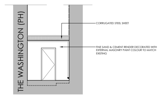
3 REAR ELEVATION PROPOSED 1:100
