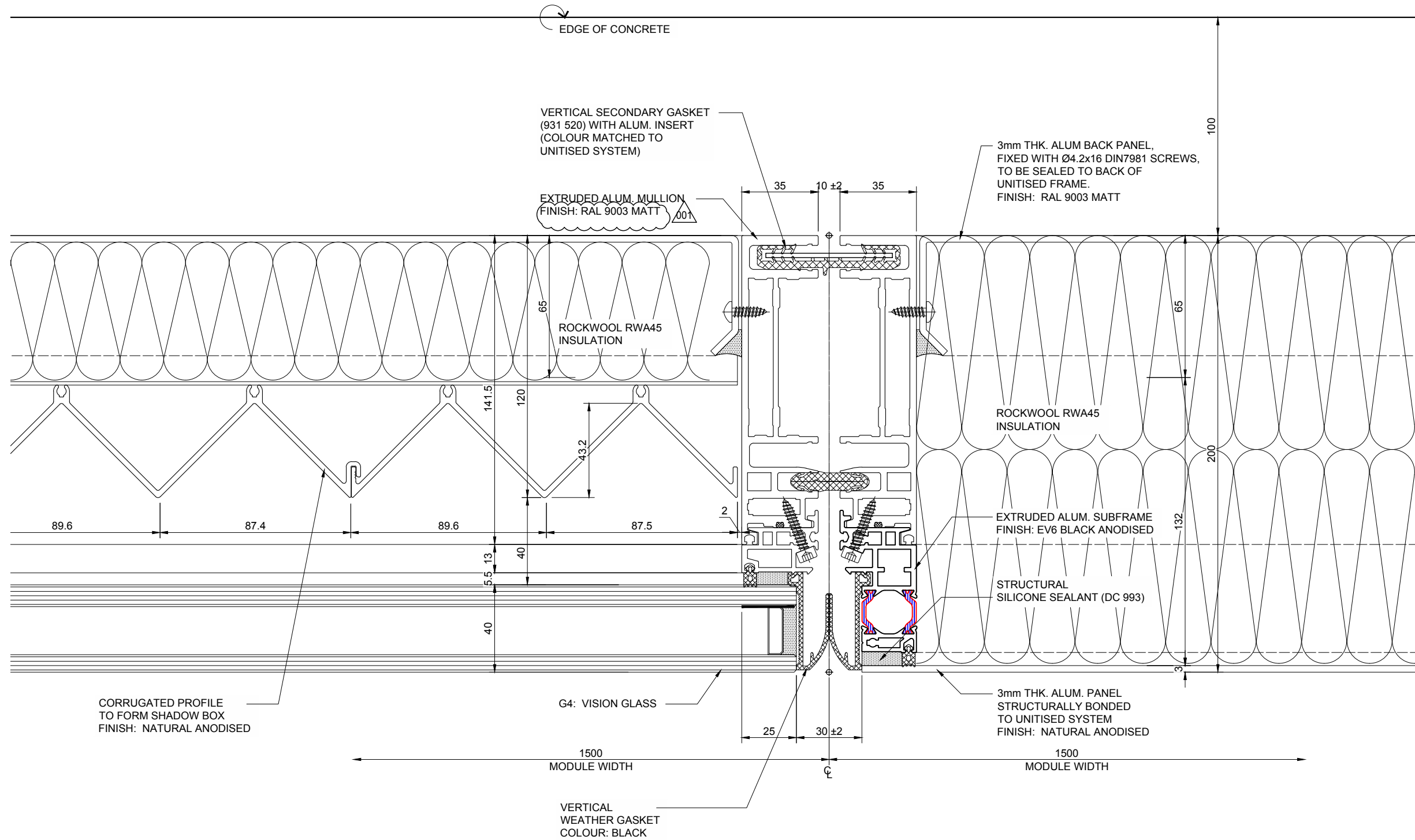
1 PLAN DETAIL Scale: 1:2
