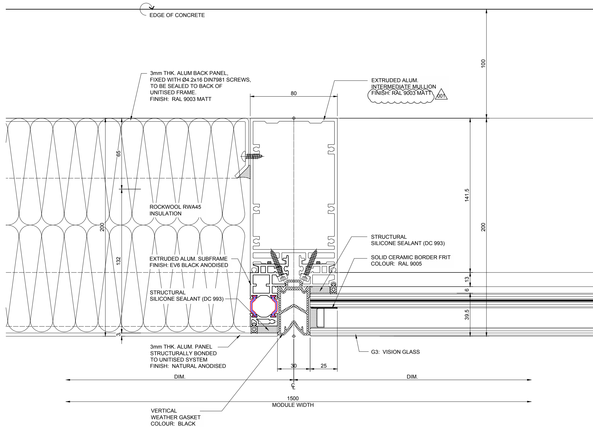
1 PLAN DETAIL Scale: 1:2
