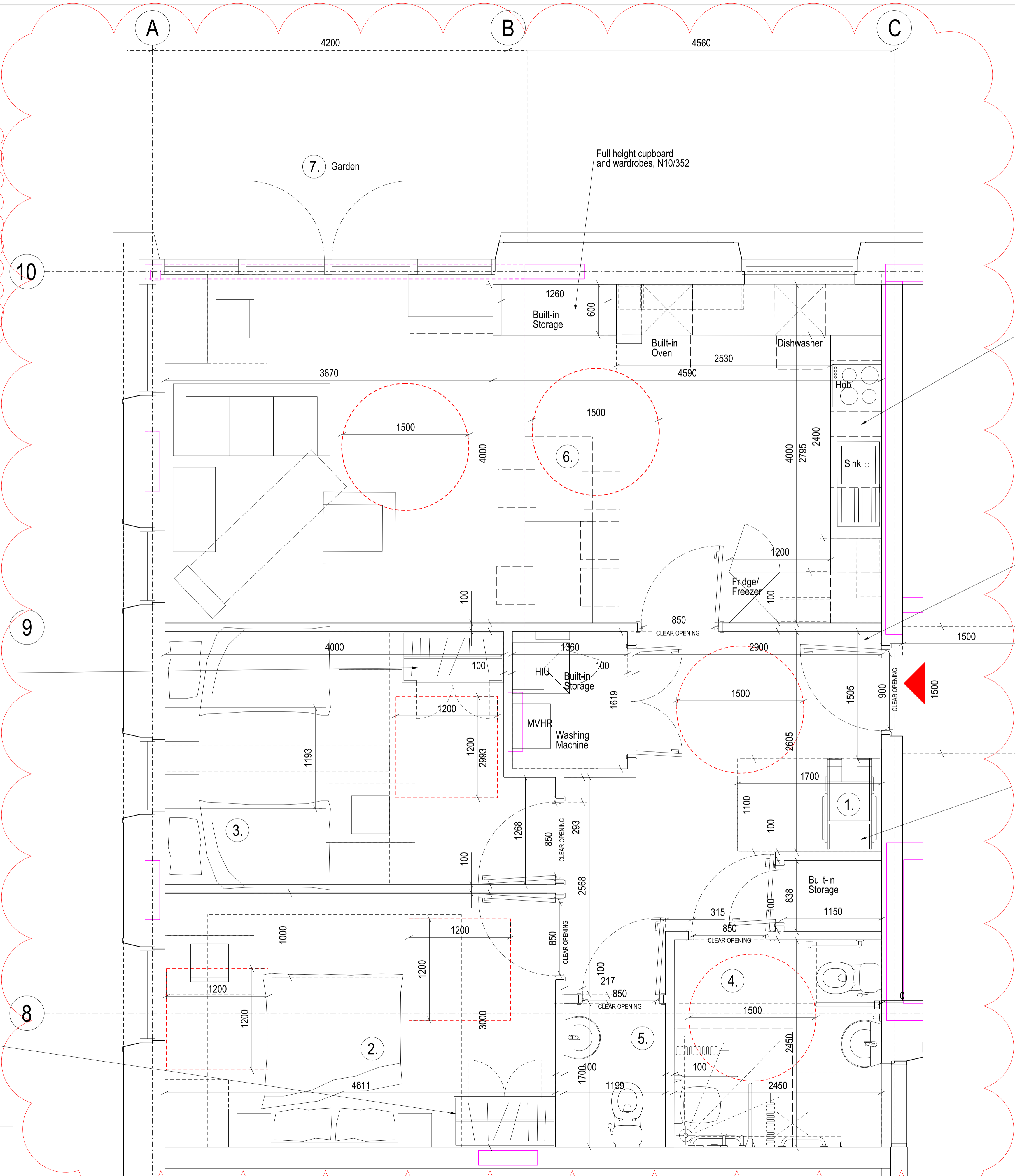
A 2 Bed - 4 Person Wheelchair Accessible Flat Plan 4540 1:25 @ A1 / 1:50 @ A3
