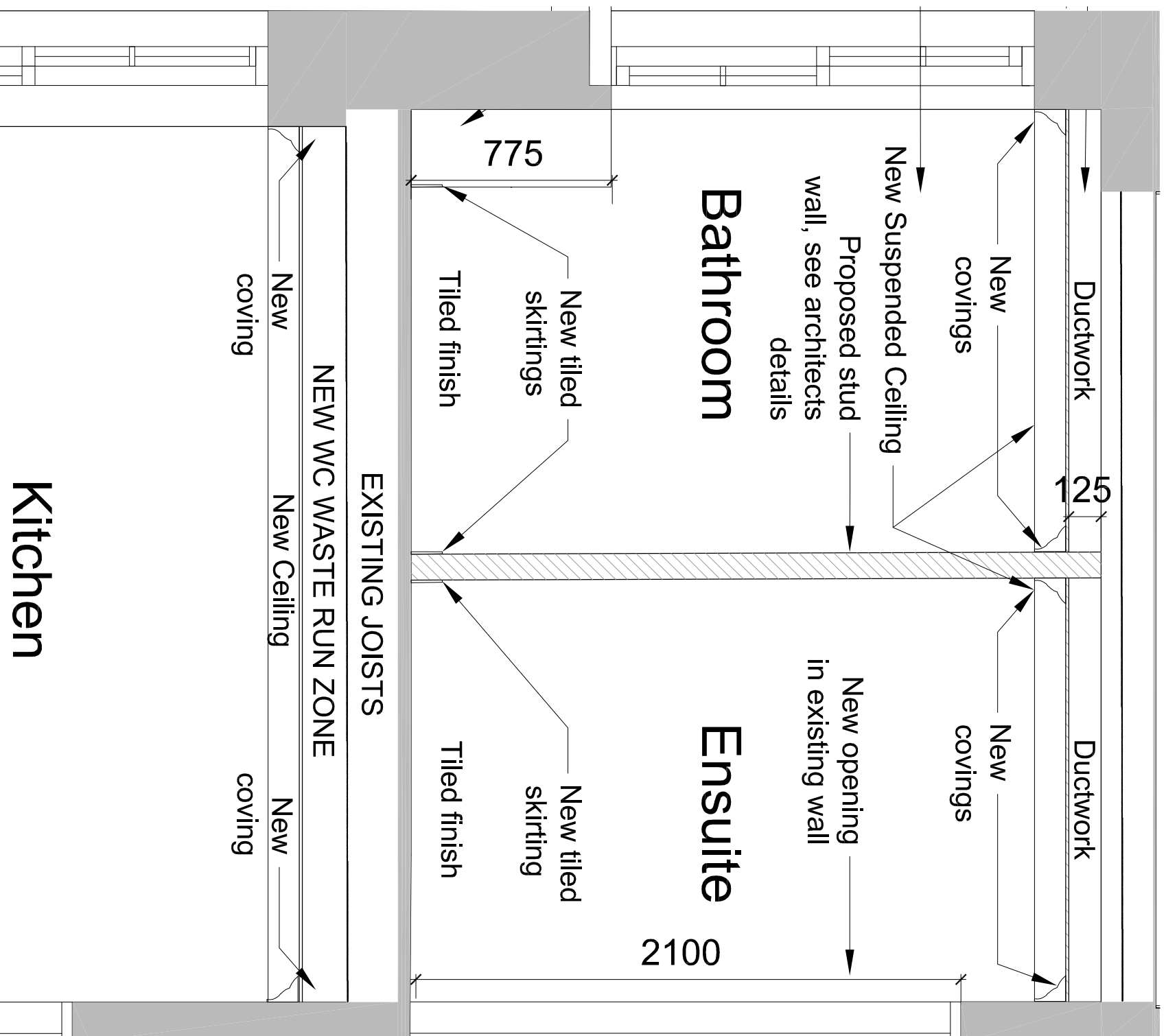
A Section through kitchen & bathroom 1:25@A1
