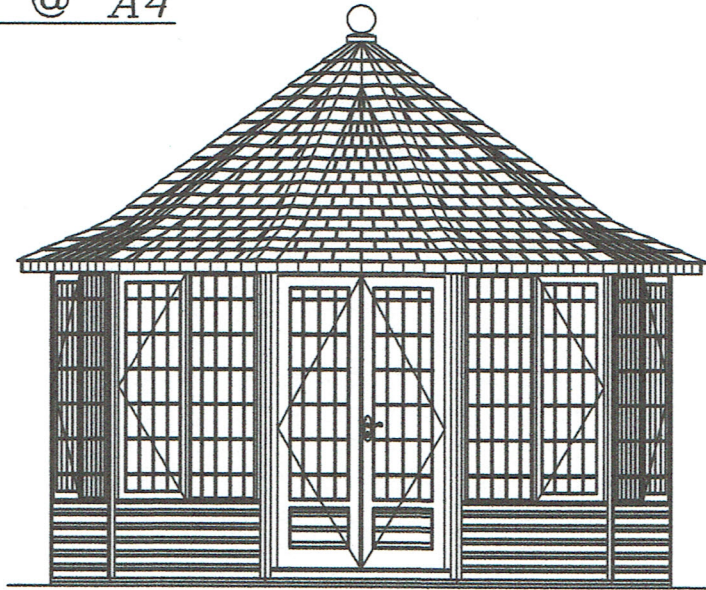
FRONT ELEVATION
