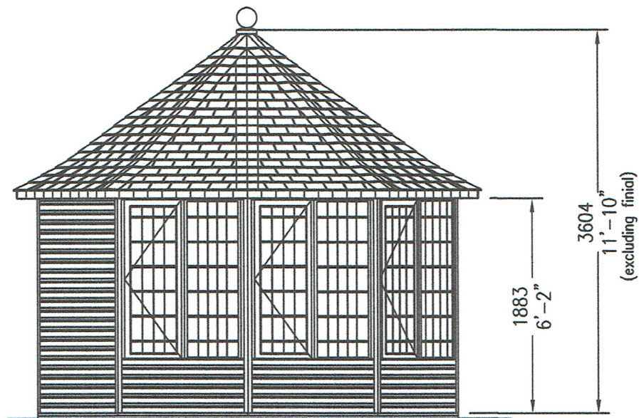
SIDE ELEVATION
