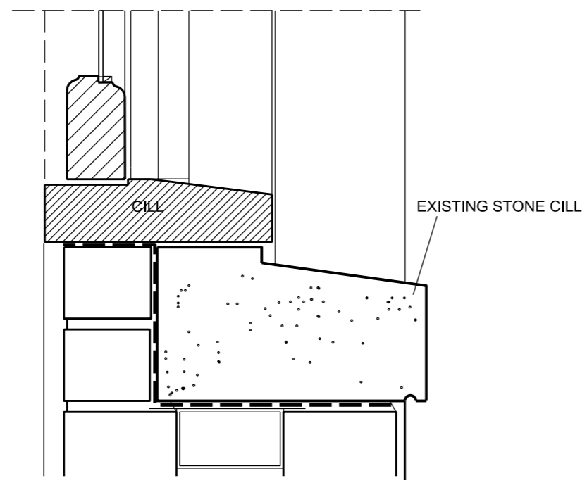
TYPICAL EXISTING SASH WINDOW DETAILS
