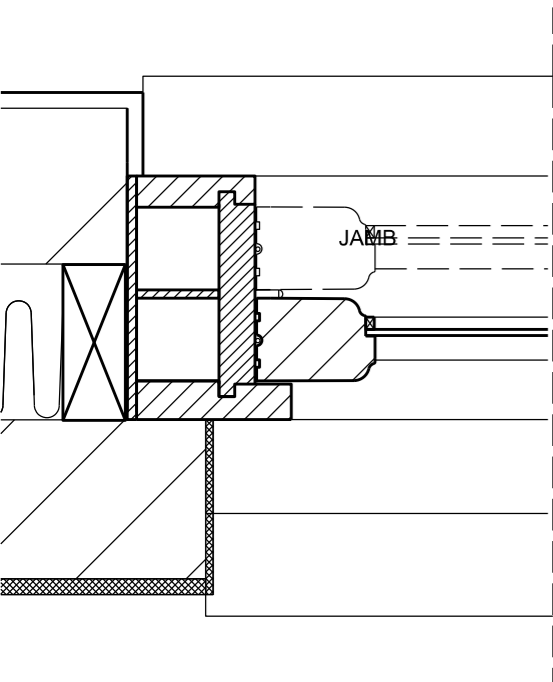
TYPICAL EXISTING SASH WINDOW DETAILS
