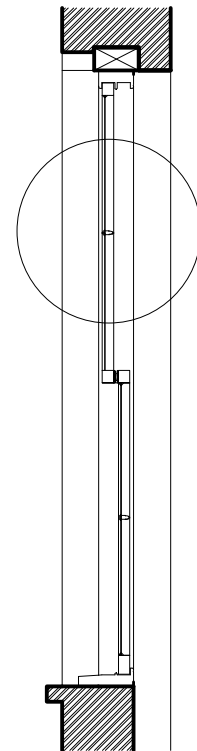
Sash Window Section Sc. 1:25
