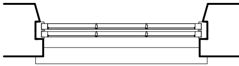
Sash Window Plan Sc. 1:25
