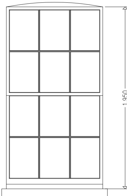
Sash Window Elevation Sc. 1:25
