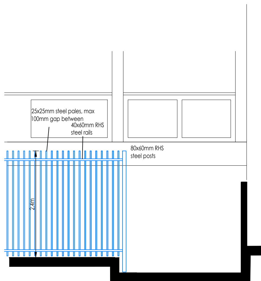
FRONT ELEVATION ENTRANCE GATE
