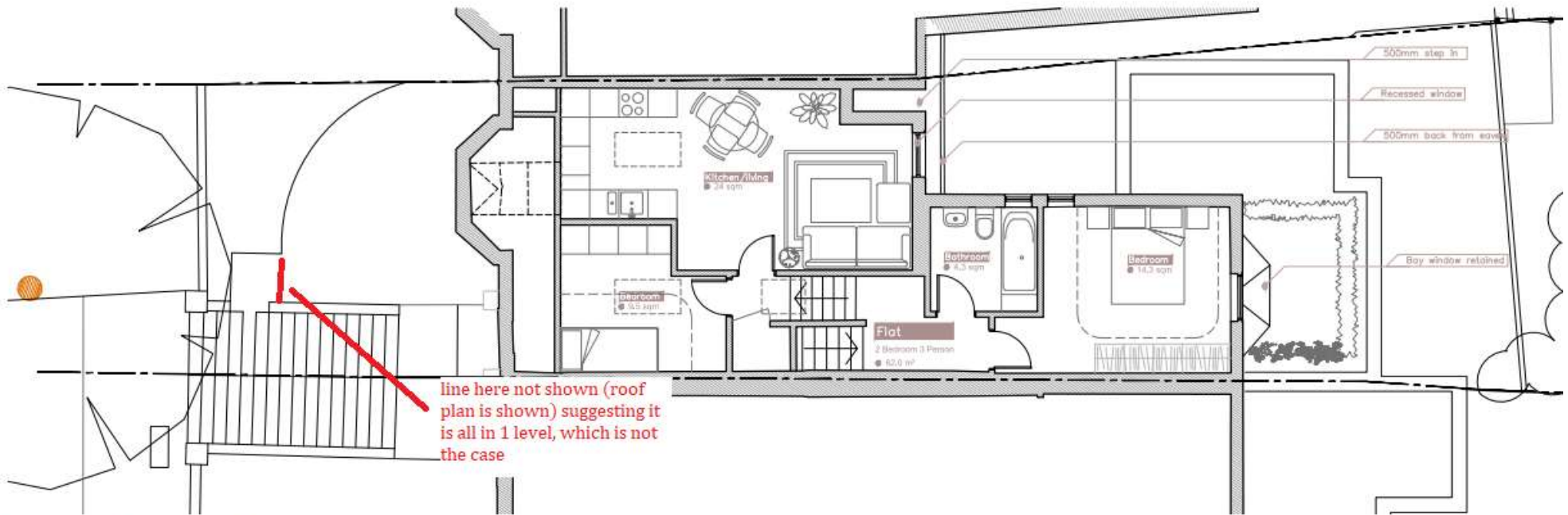
Proposed Second Floor Plan - 1:100@A3
