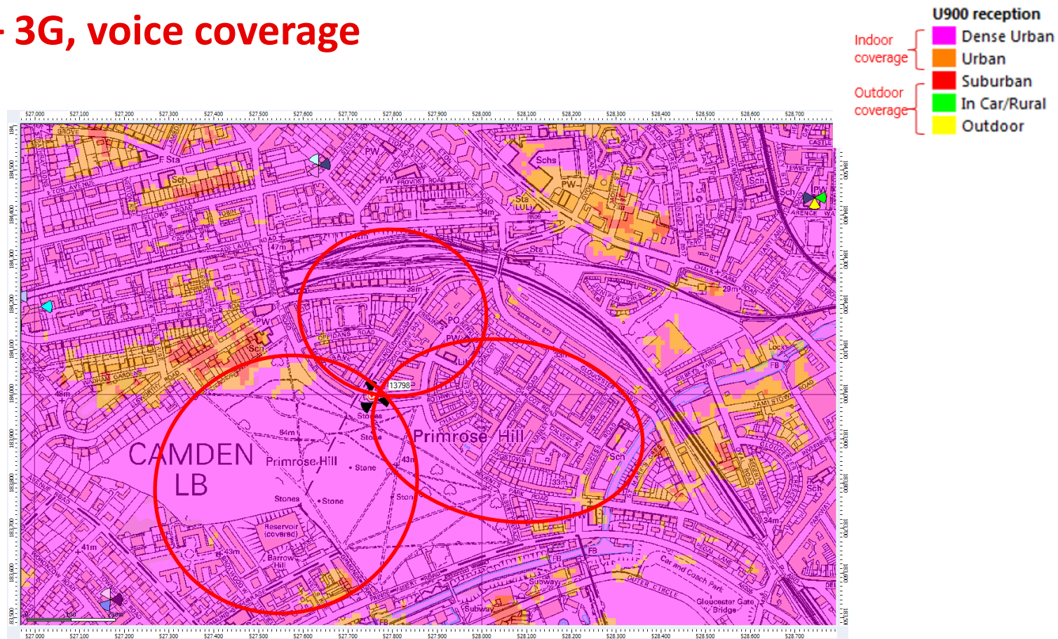
Fig. 4: Proposed UMTS900MHz, (new site 13798)
