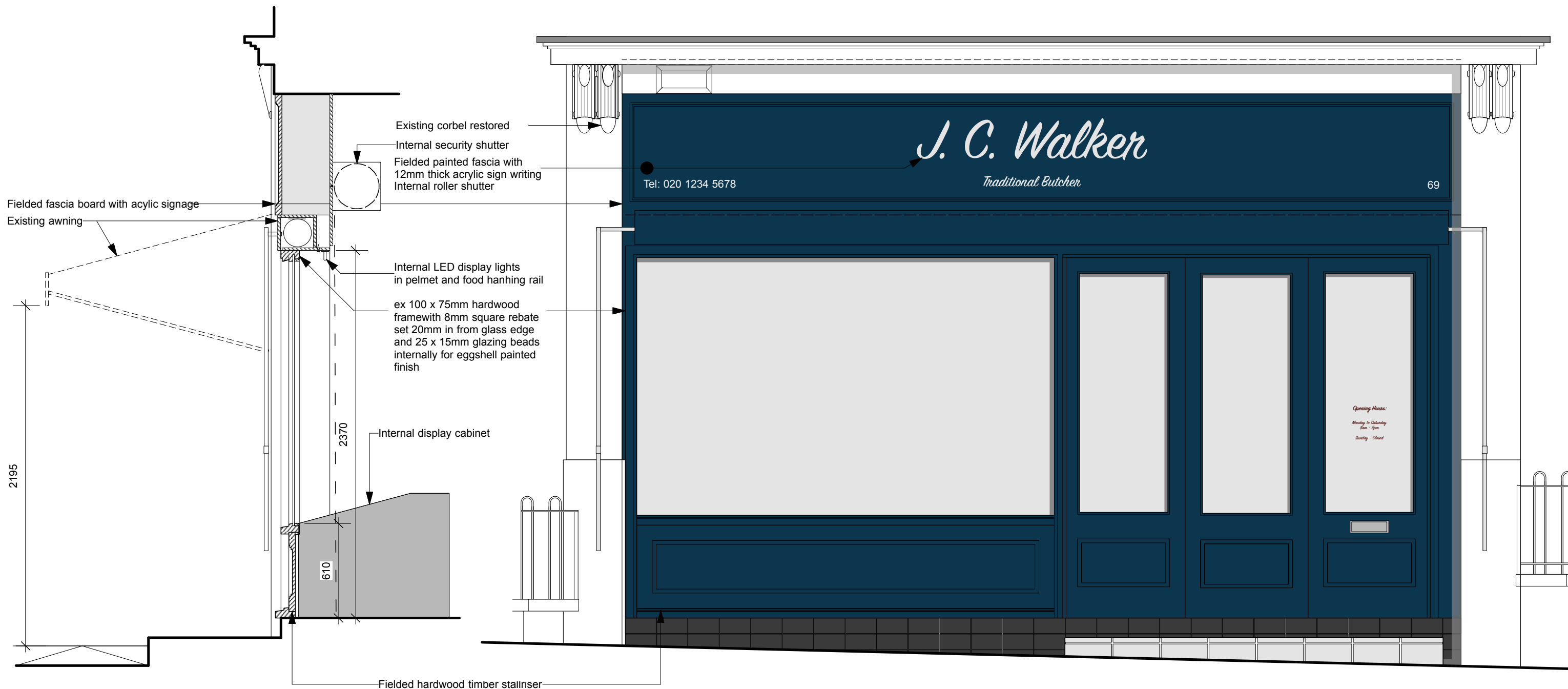
Section Through Shopfront 1:25 scale
