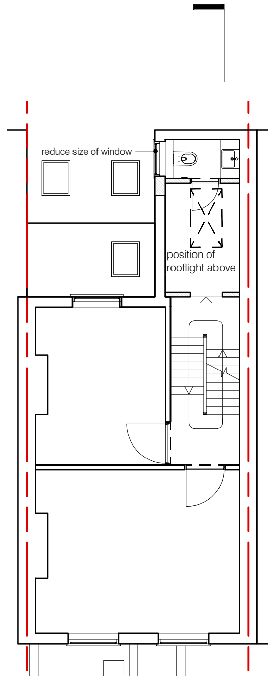
01 PROPOSED FIRST FLOOR PLAN scale 1:100
