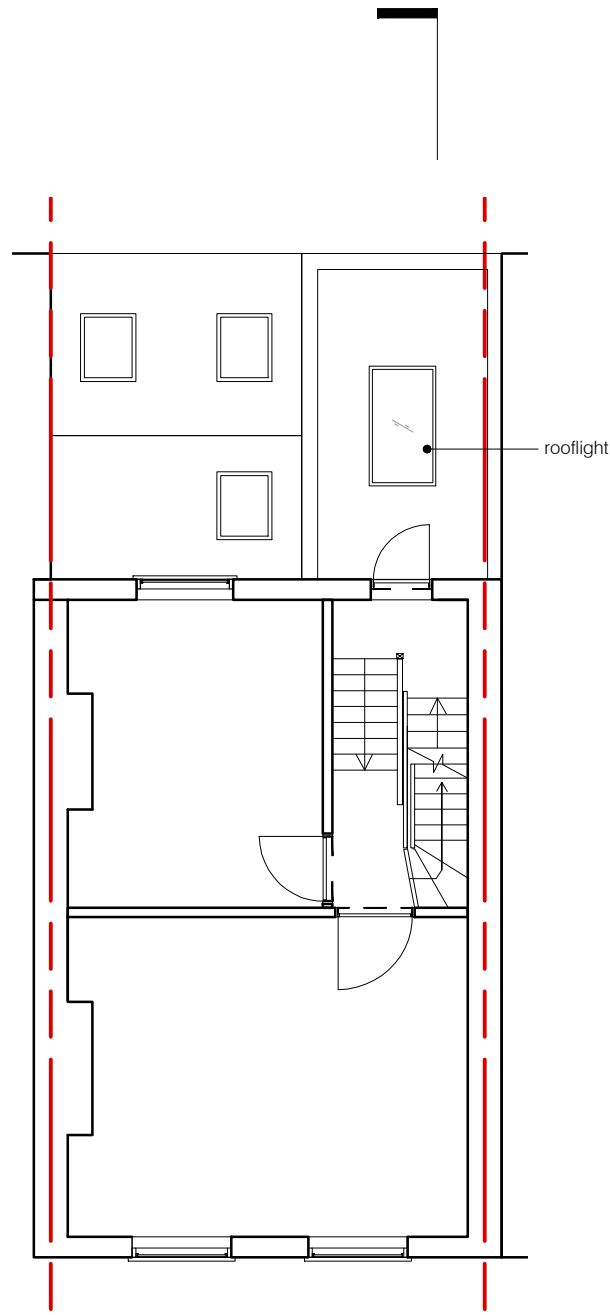
02 PROPOSED SECOND FLOOR PLAN scale 1:100
