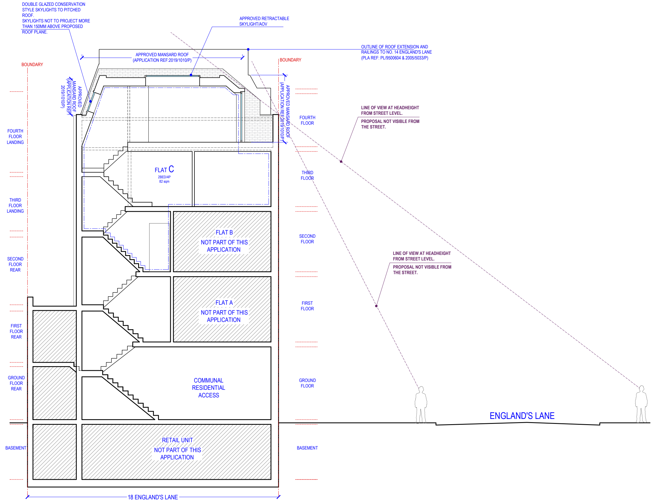
[01] APPROVED SECTION 'AA' : 2019/1010/P @1:100
