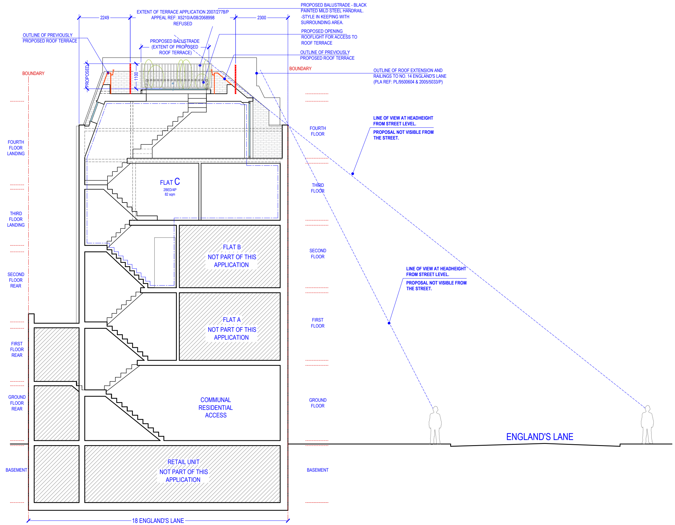
[01] PROPOSED SECTION 'AA' @1:100
