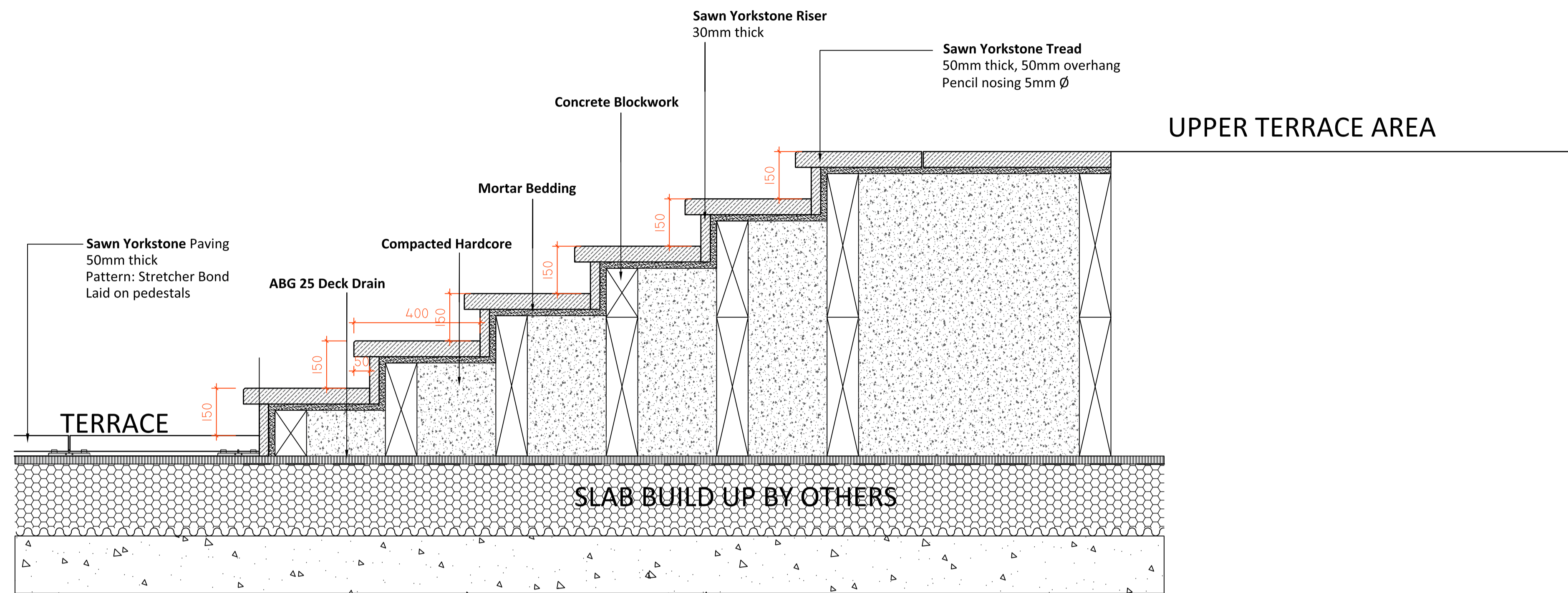
A REAR TERRACE STEPS DETAIL
