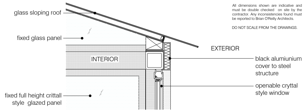
03 DETAIL 1 scale 1:10
