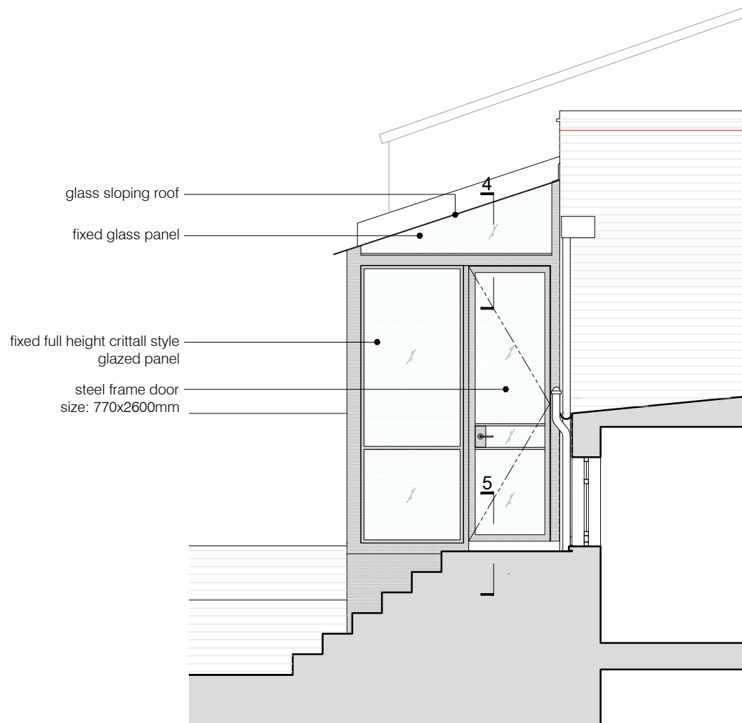
02 PROPOSED SIDE ELEVATION scale 1:50
