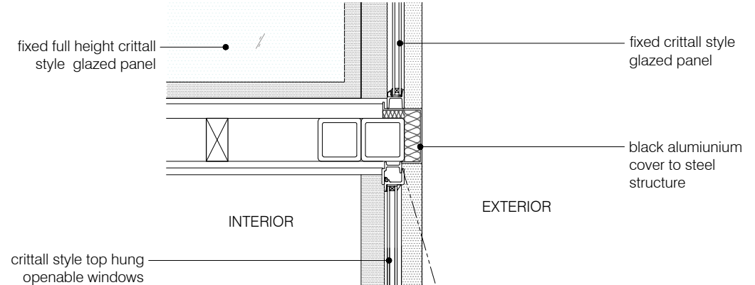
04 DETAIL 2 scale 1:10
