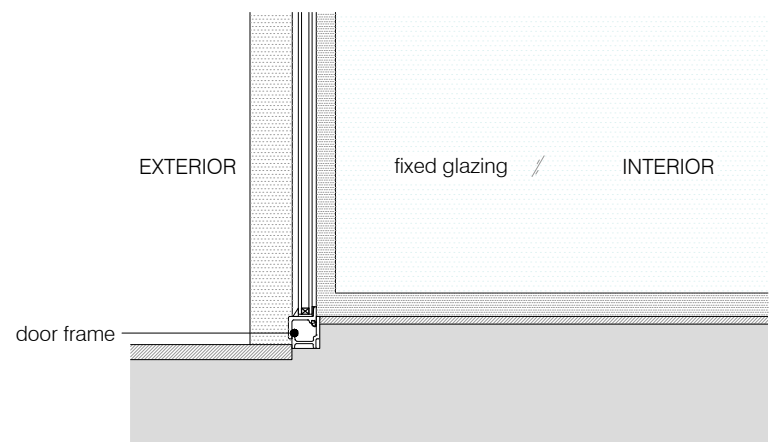
07 DETAIL 5 scale 1:10
