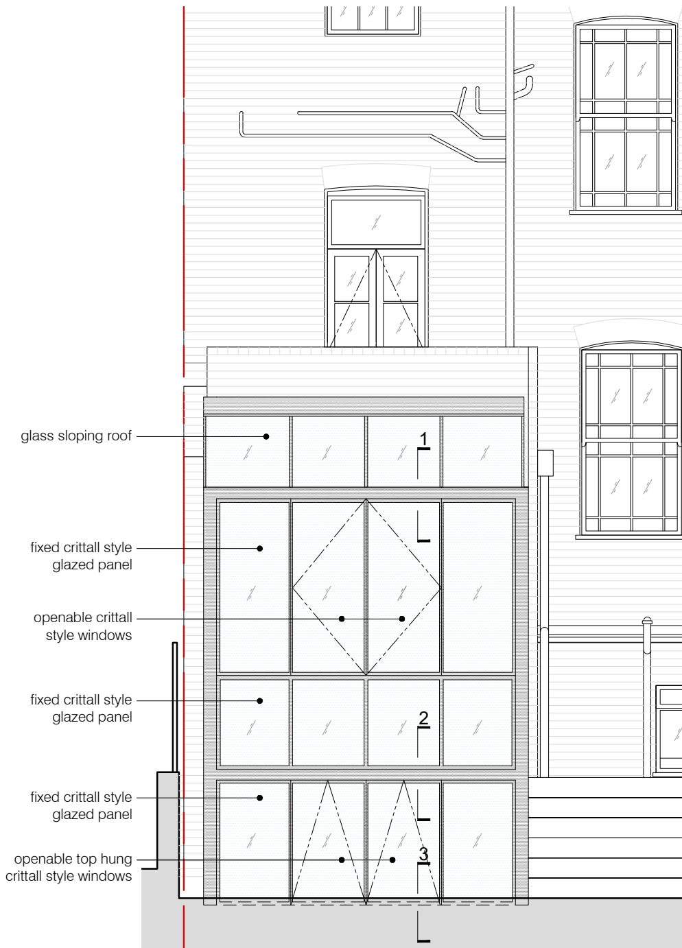
01 PROPOSED REAR ELEVATION scale 1:50
