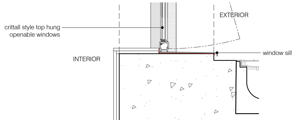
05 DETAIL 3 scale 1:10
