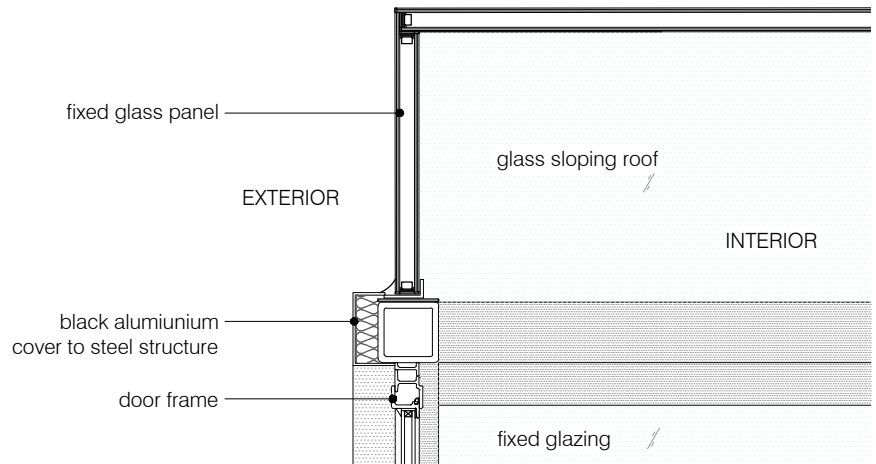
06 DETAIL 4 scale 1:10
