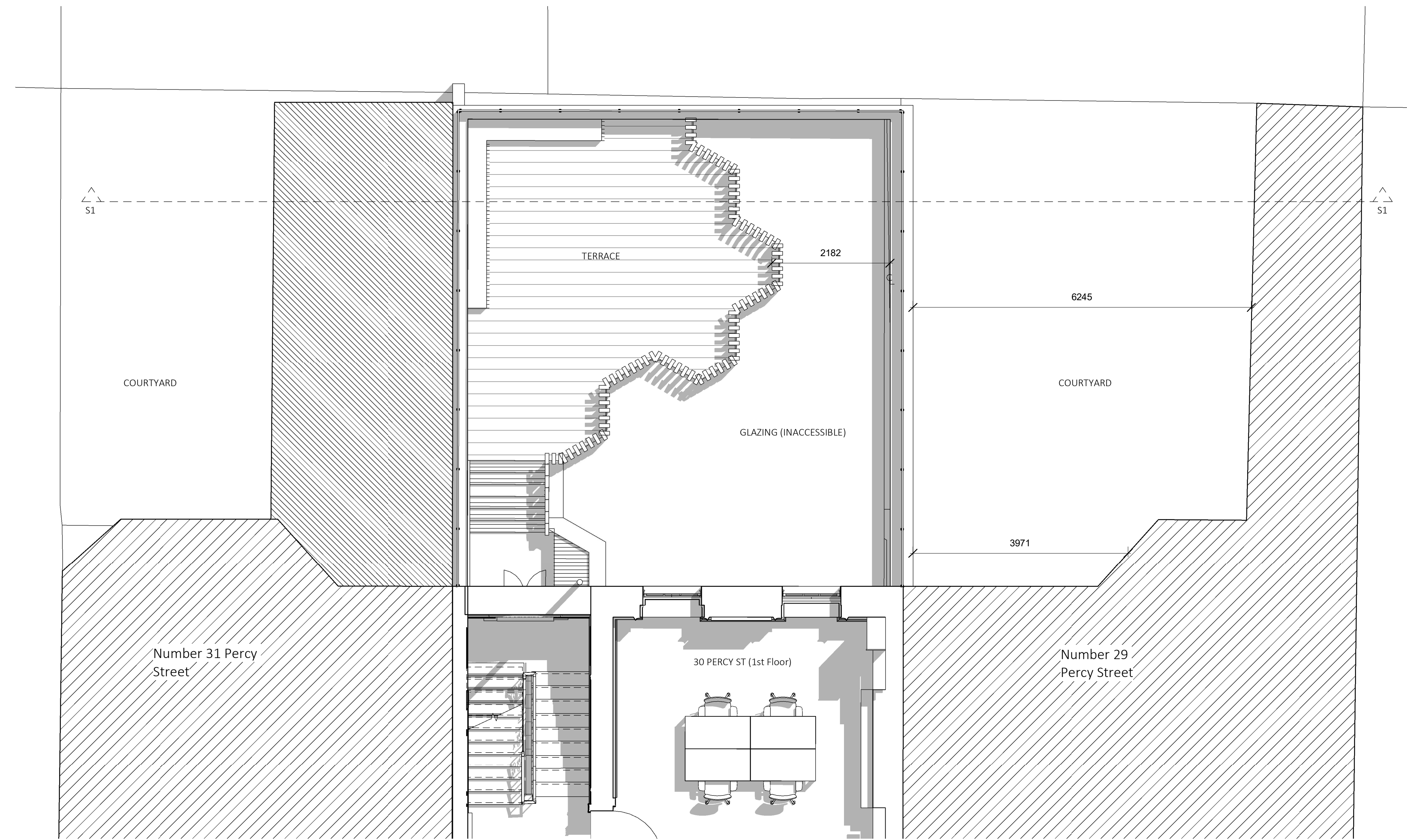
1 Proposed Level 01 1 : 50
