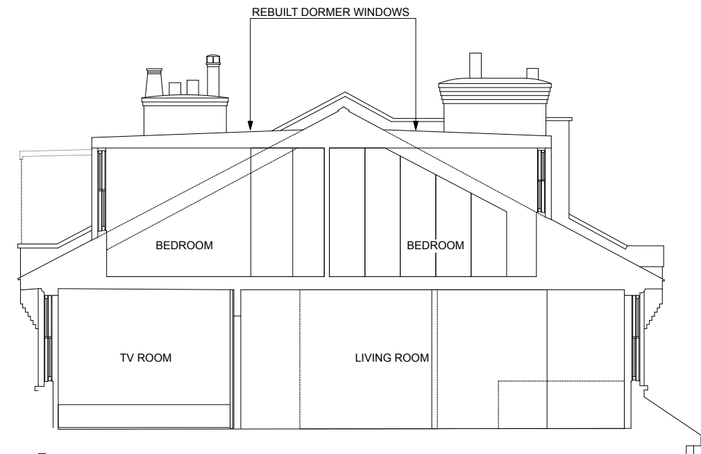
PROPOSED SECTION B
