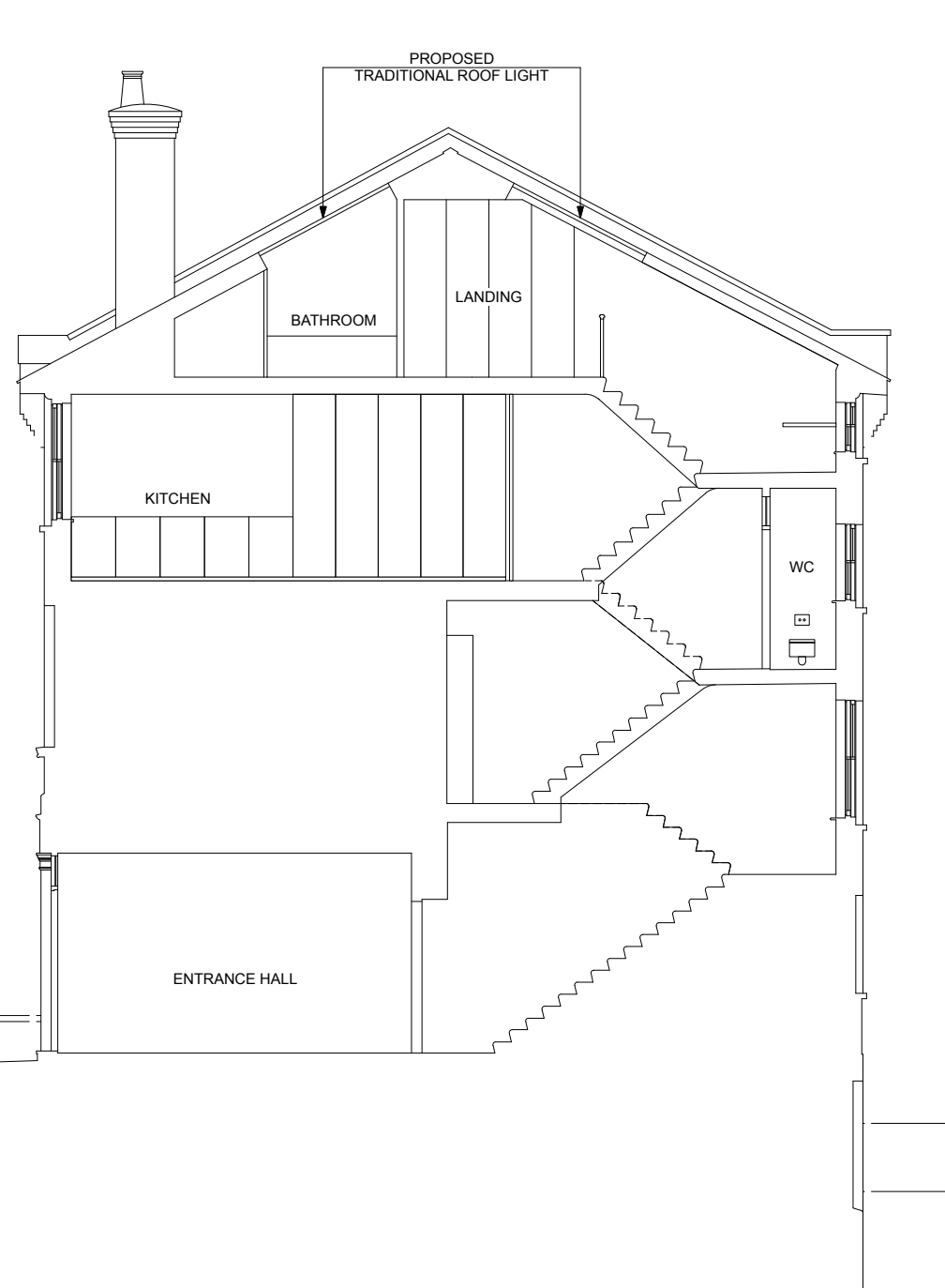
PROPOSED SECTION A (THROUGH ENTRANCE STAIR)
