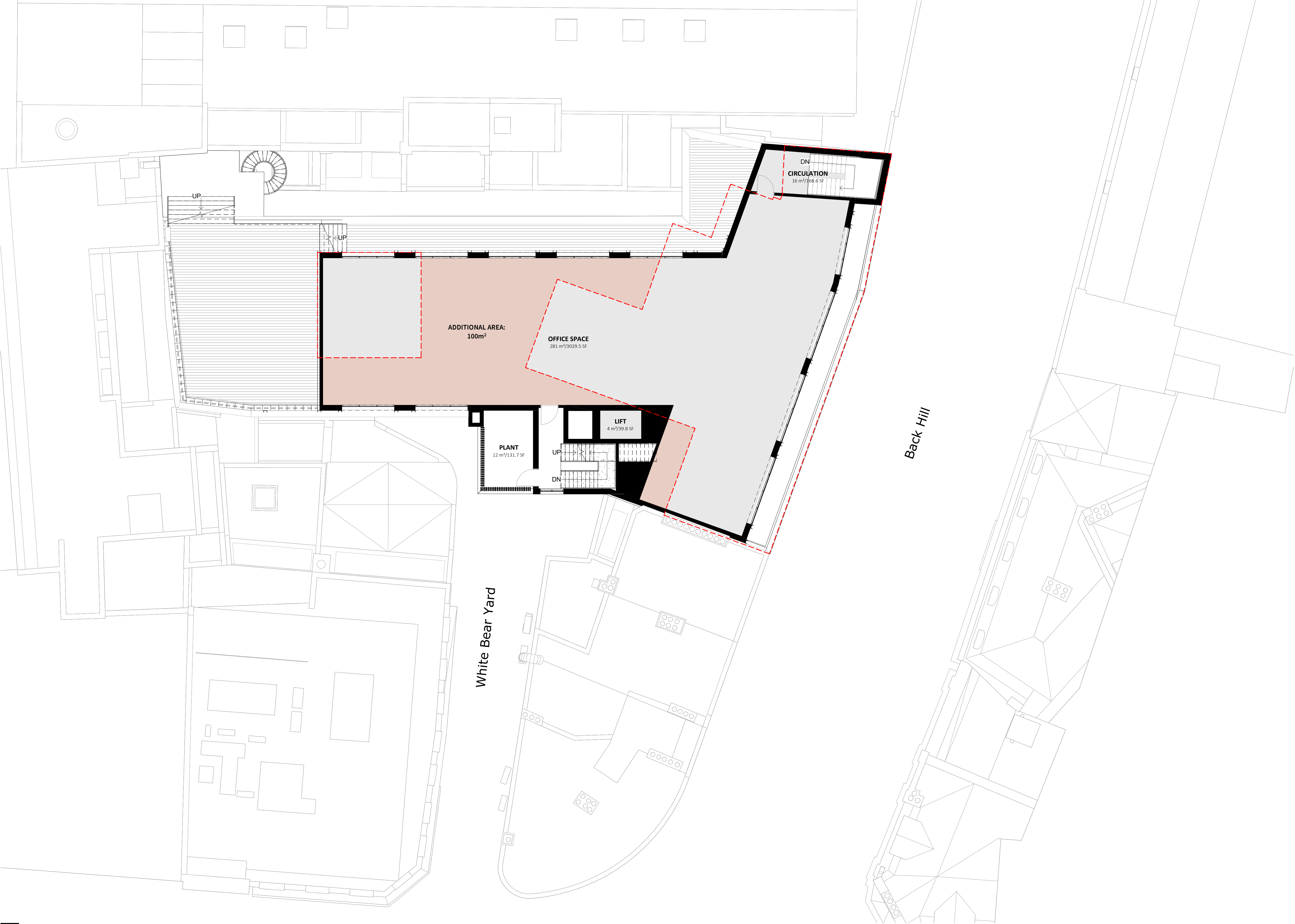
03 Proposed Third Floor Plan
