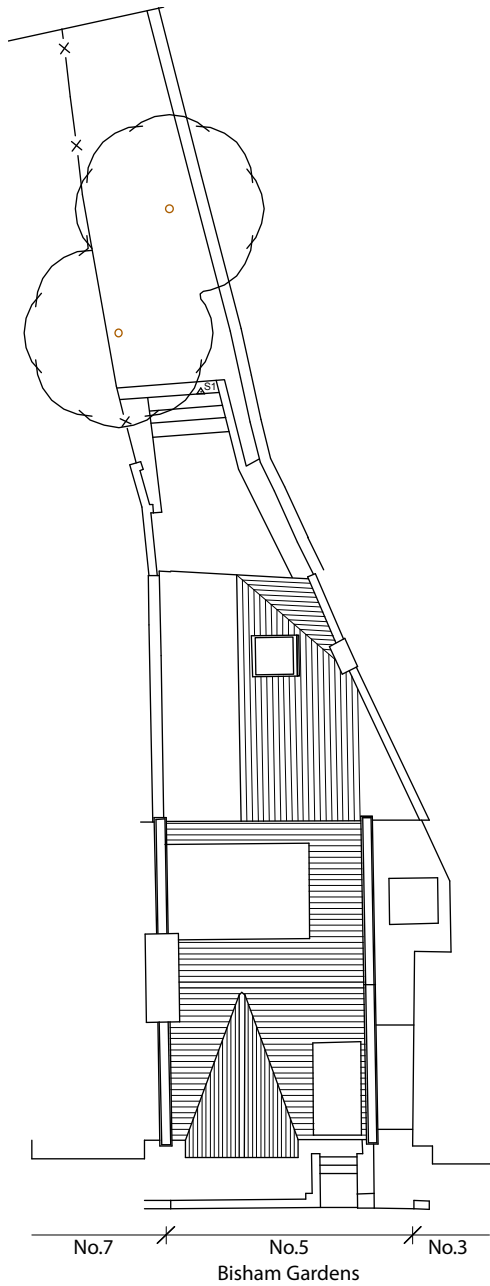
Proposed Site Block Plan
