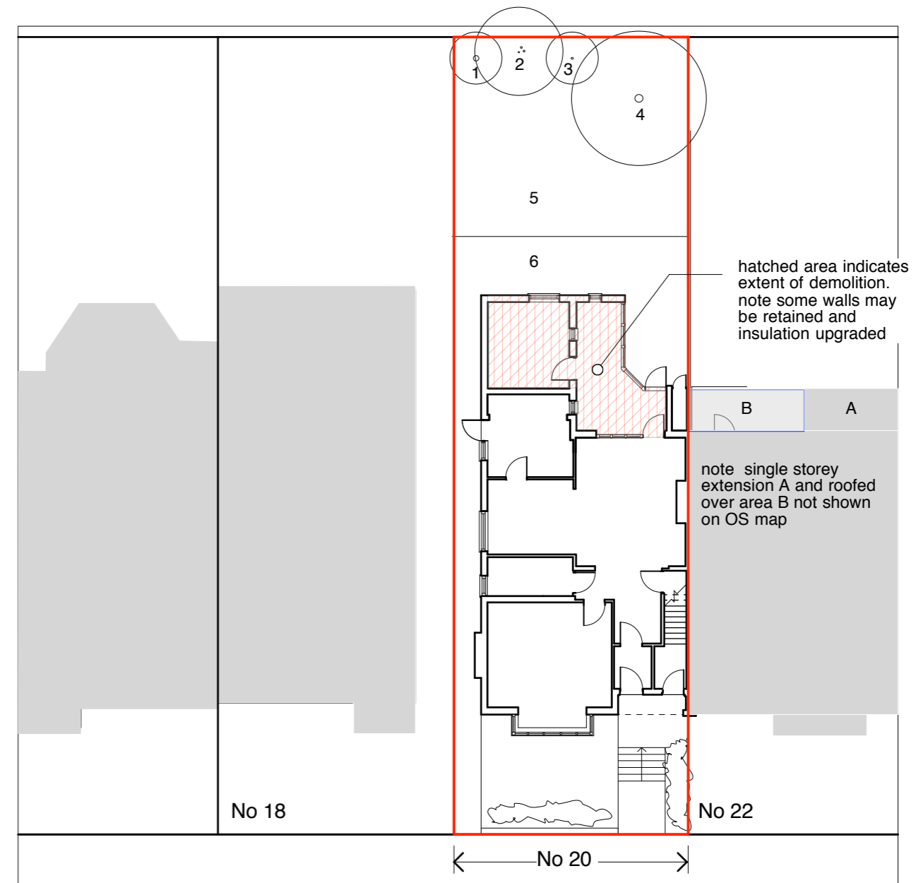
site plan - 1:200 existing
