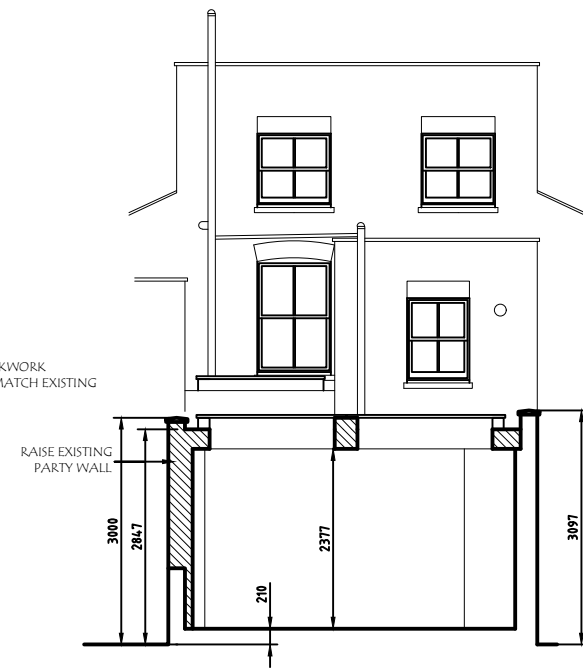
PROPOSED SECTION A-A
