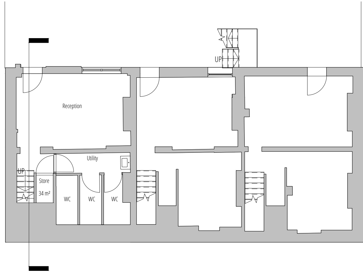
1 Existing Lower Ground Floor GA Plan 1:100
