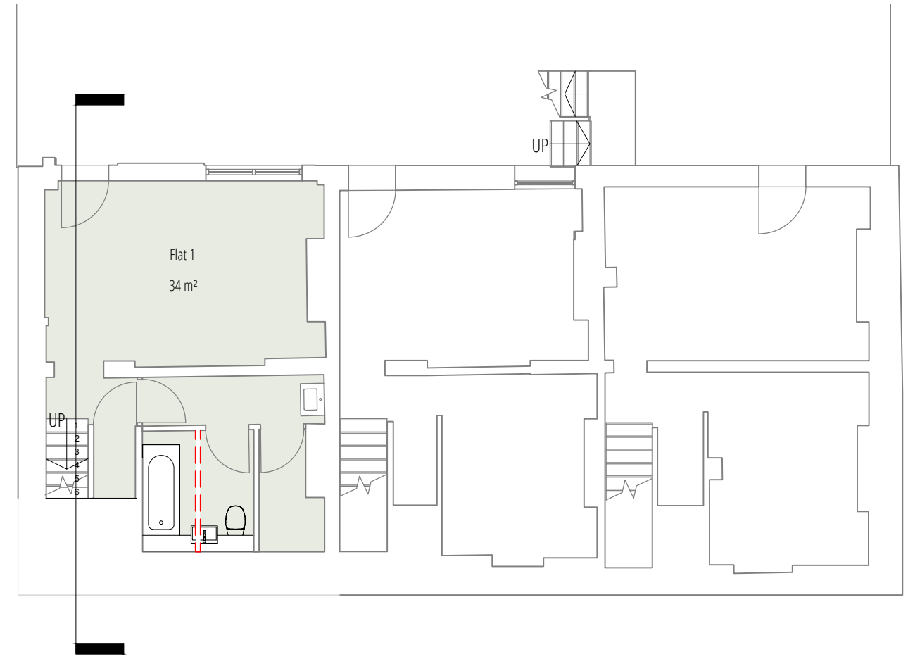
2 Proposed Lower Ground Floor GA Plan 1:100
