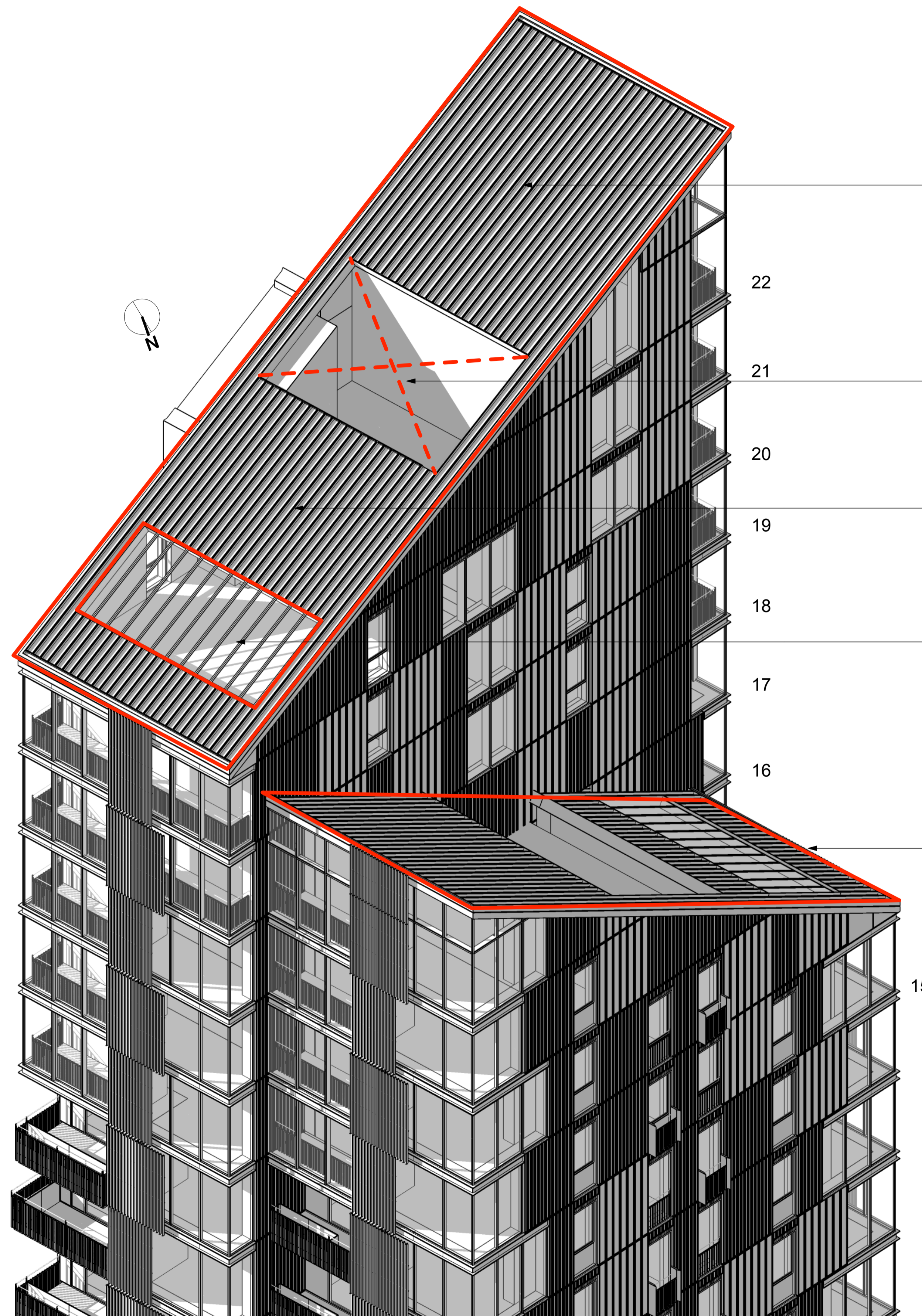
1 ISOMETRIC VIEW
