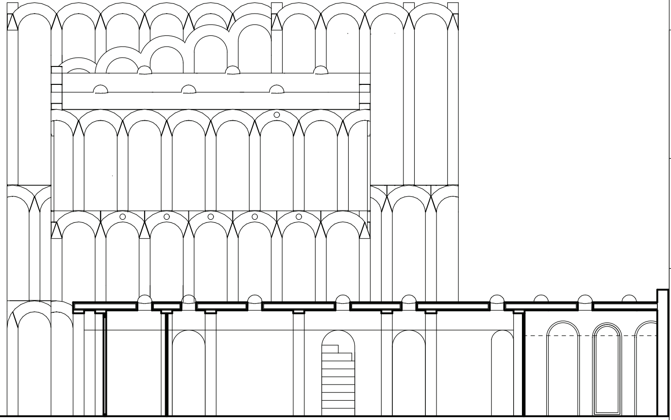
PROPOSED EAST ELEVATION 1:100
