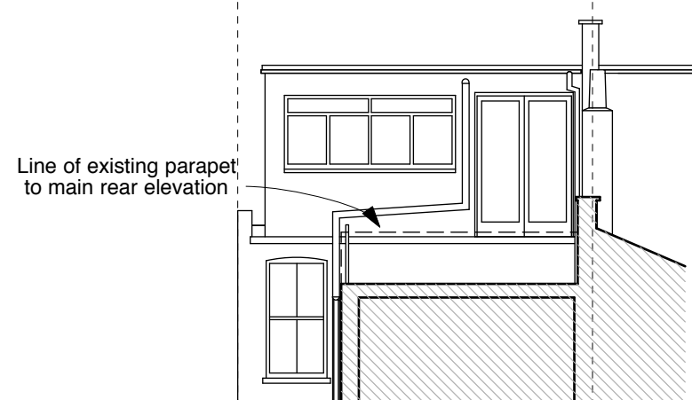
Existing Part Section A-A
