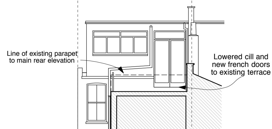
Proposed Part Section A-A
