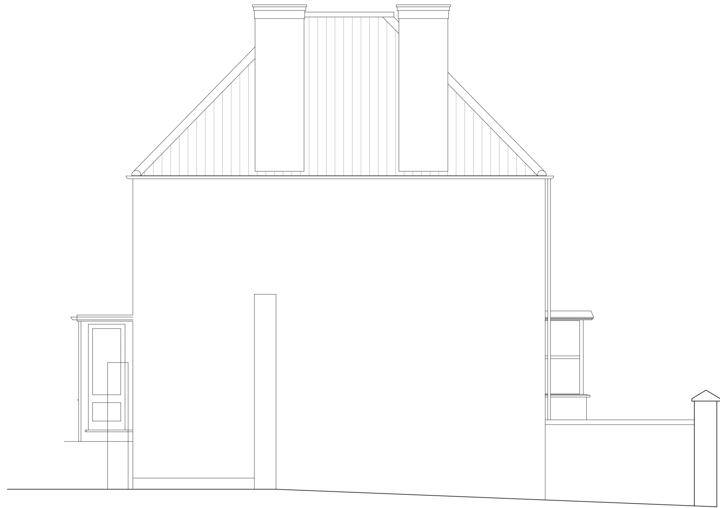
4 east/side elevation
