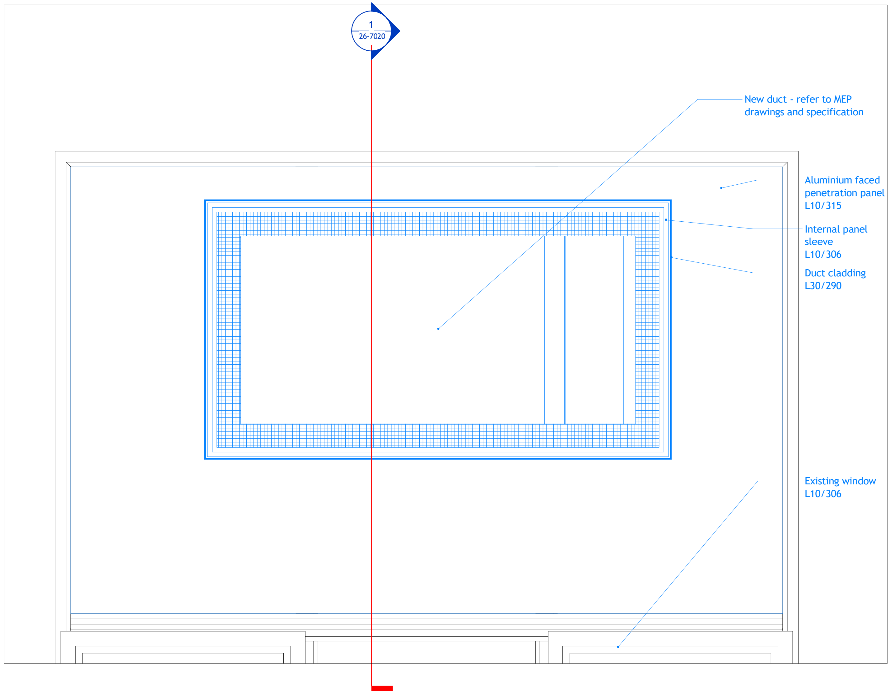
2 Window Services Penetration Panel - Detail Elevation 1 : 5
