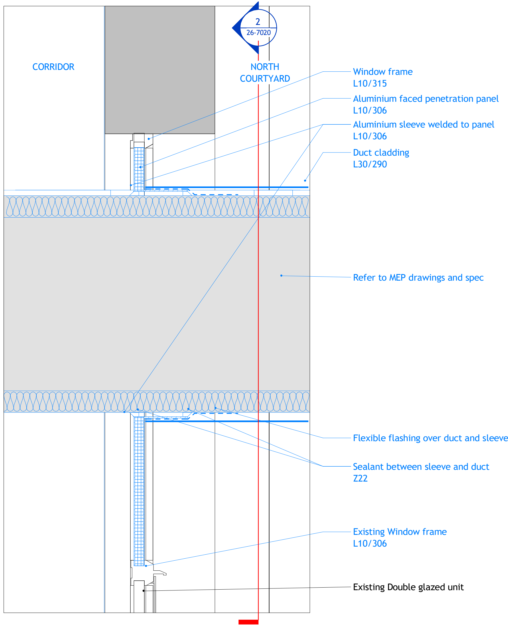
1 Window Services Penetration Panel - Detail Section 1 : 5
